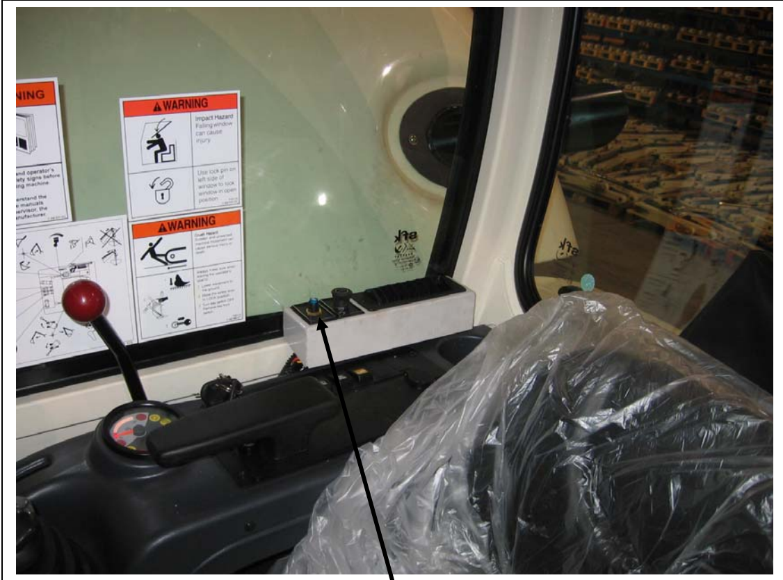
A 72" rotary thermostat is mounted at this location in place of the push button.
